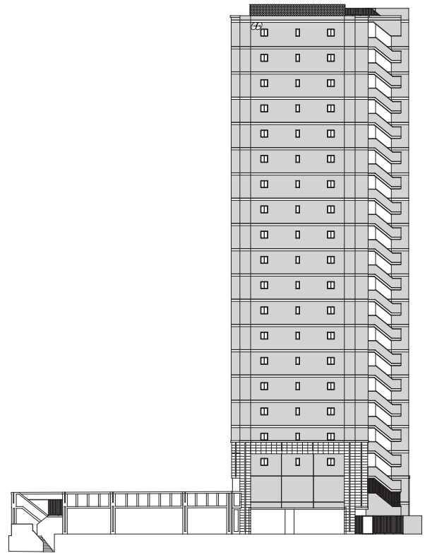
●東側立面图 EAST SIDE VIEW
